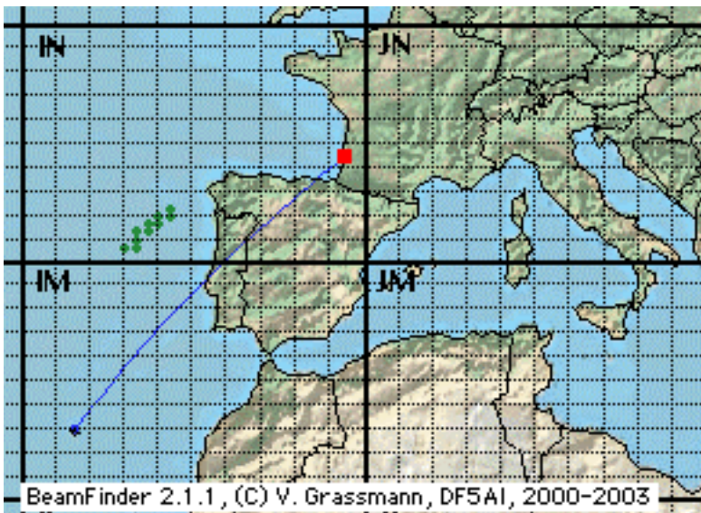
FAI scatter volumes (dot marks) corresponding to the path F-CT3.
